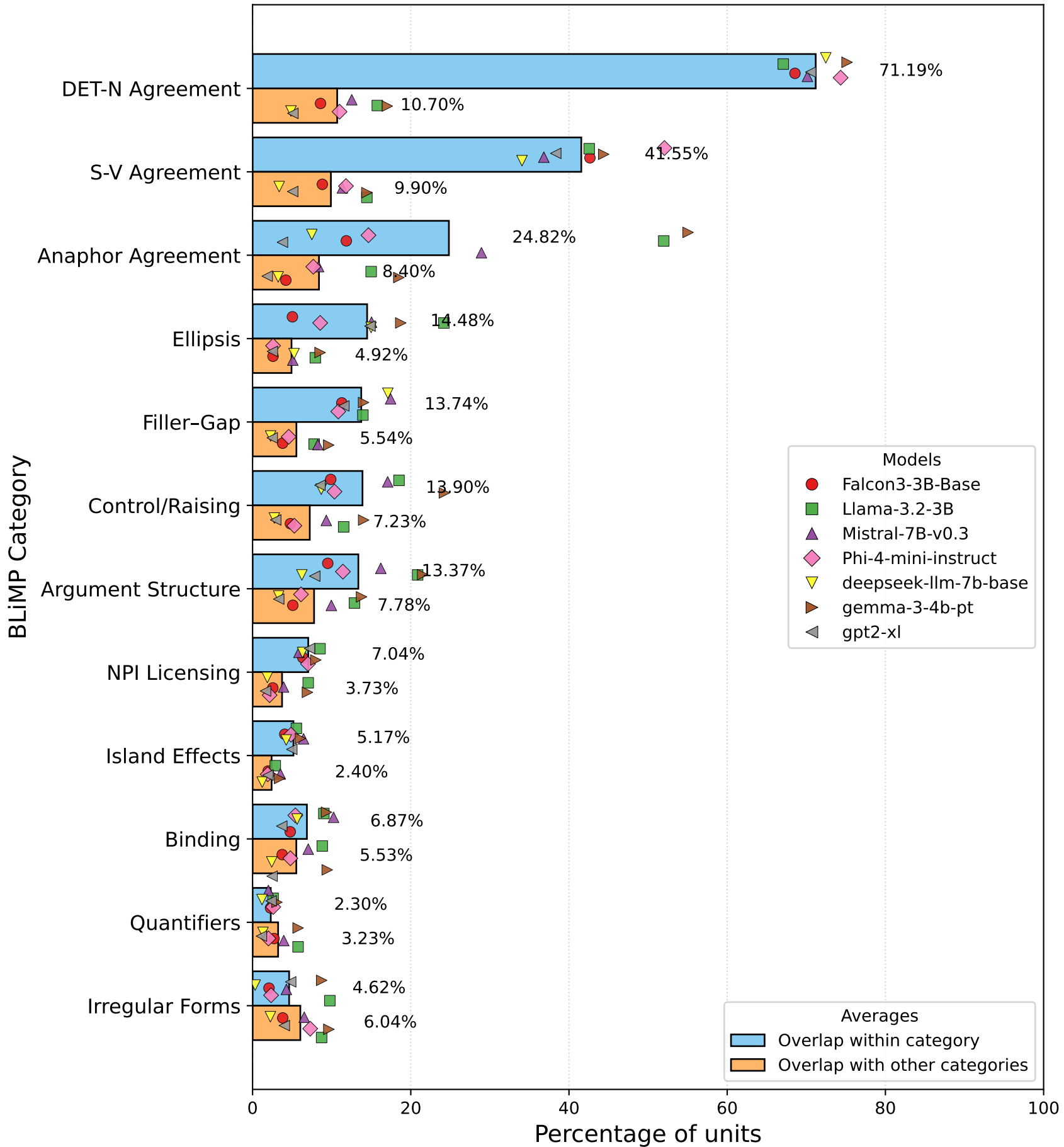
Cross-phenomenon overlap in BLiMP across seven models
